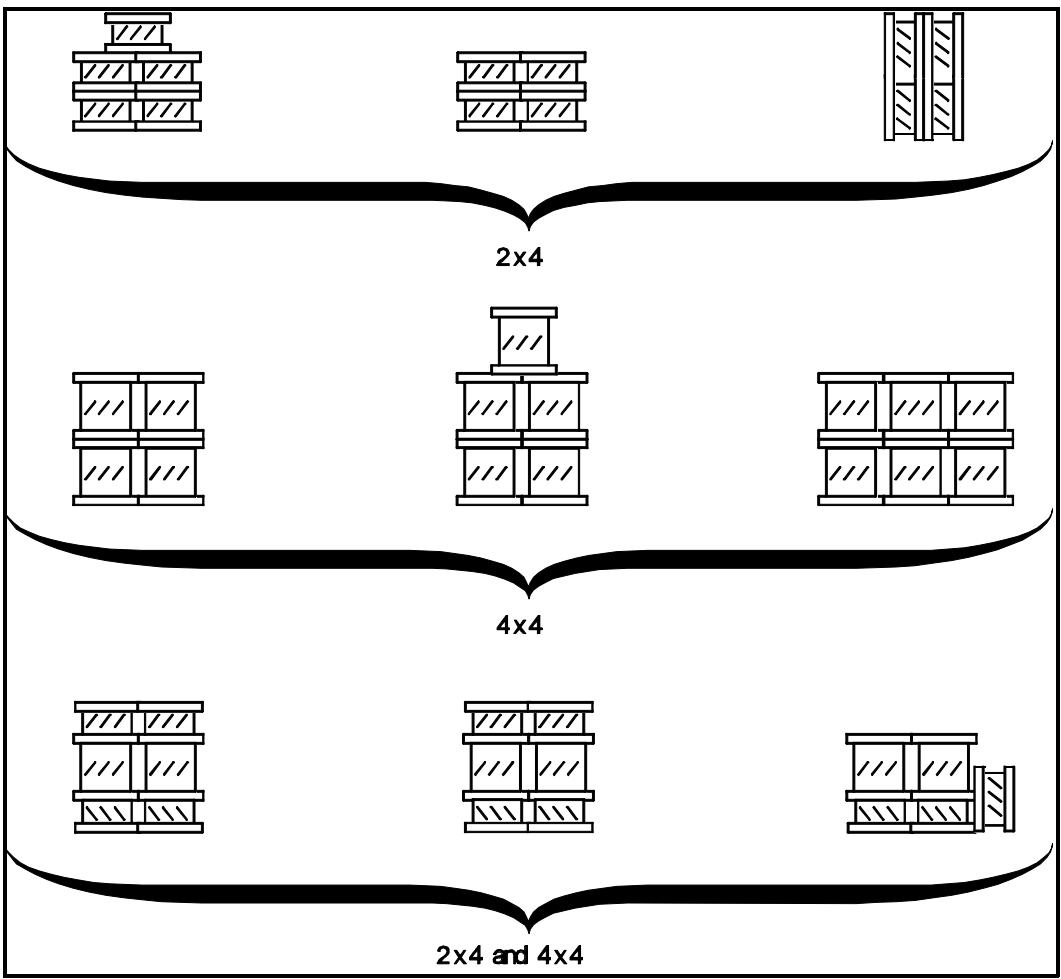
Figure 28-3. Test Fuel Crib Arrangements.
