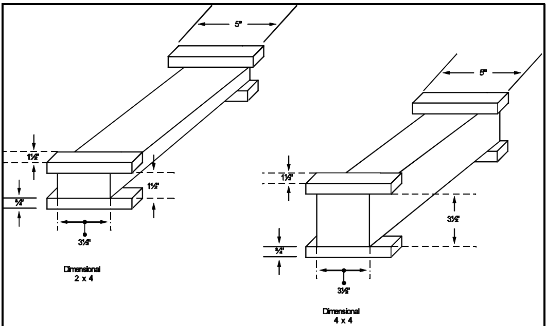
Figure 28-2. Test Fuel Spacer Dimensions.
